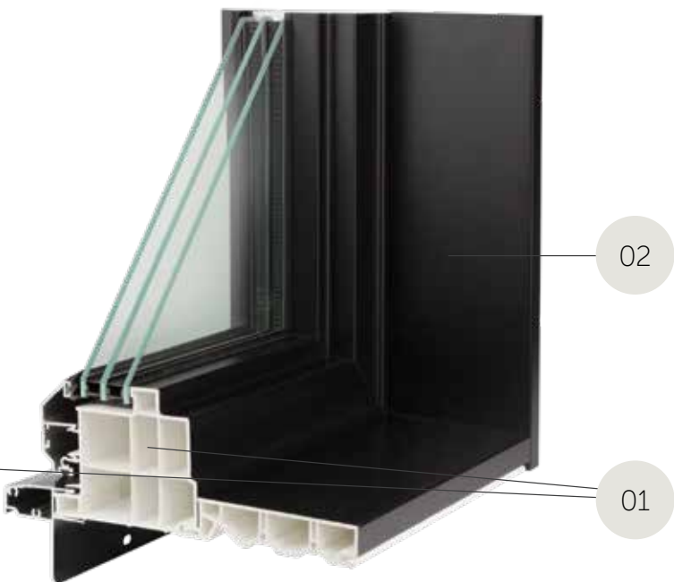
Hybrid Fixed Sash with uPVC nite Jamb Extension
